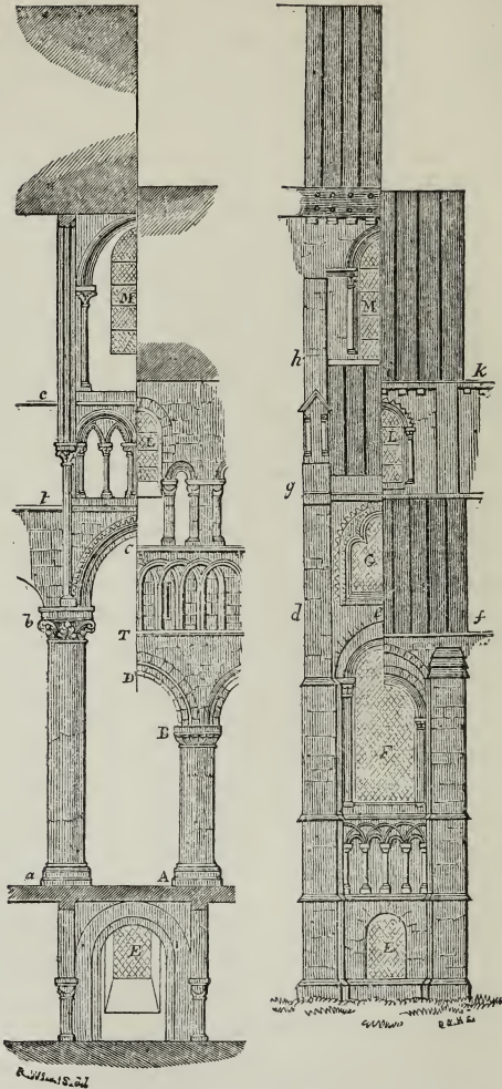
71. Canterbury Cathedral.
